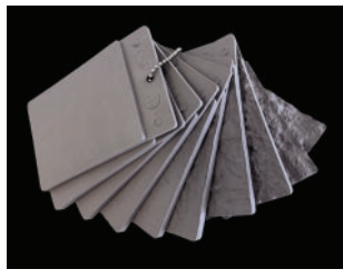
ICRI PROFILE PLASTIC CHIPSET 546 2169-02
